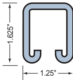
Rail RAIL SECTION 1.625" x 1.25"
